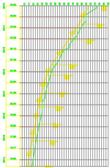
COLECTORA EC-1
